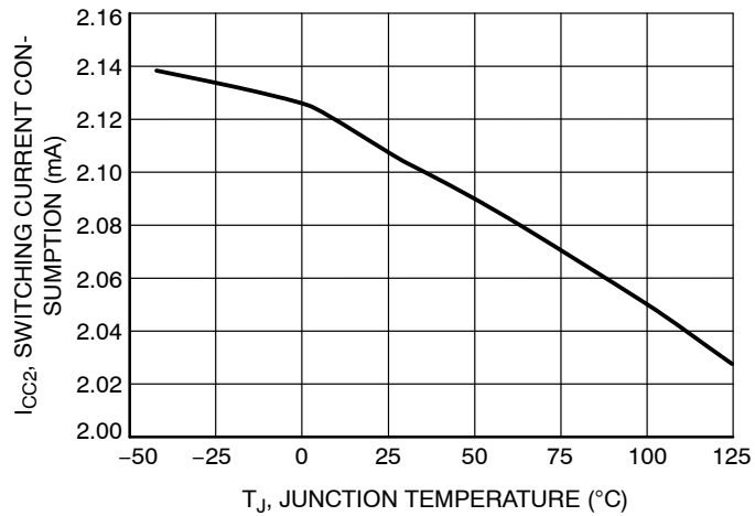
Figure 22. Switching Current Consumption vs. Junction Temperature
